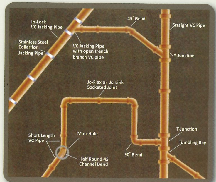
Overview of the piping system
