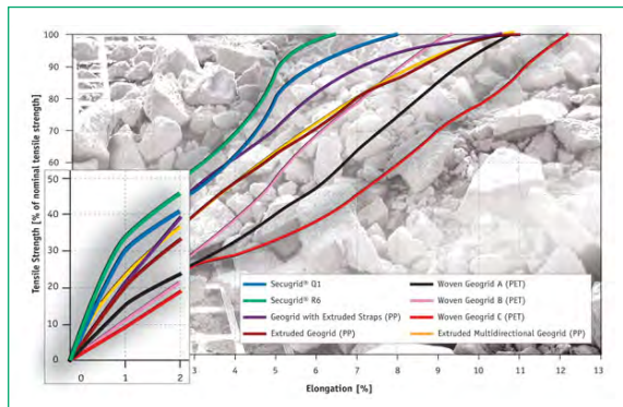
Fig. 13 Stress/strain curves of Secugrid® and selected geogrids
