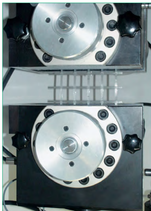
Fig. 12 Tensile strength testing of Secugrid®
