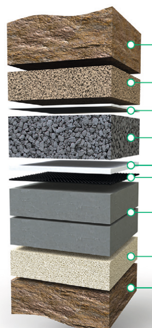
Figure 2 Intermediate sealing system for municipal solid waste landfills
