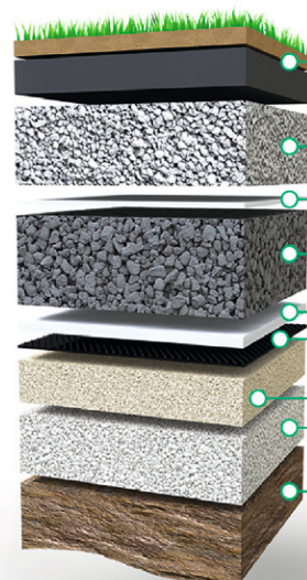
Figure 4 Cap/closure system over contaminated material to allow a future re-use of the site
