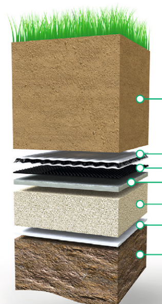
Figure 3 Cap/closure system for municipal solid waste landfills
