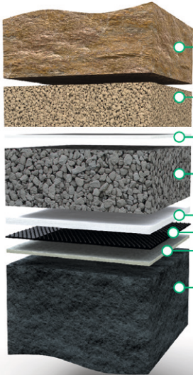
Figure 1 Base sealing system for municipal solid waste landfills
